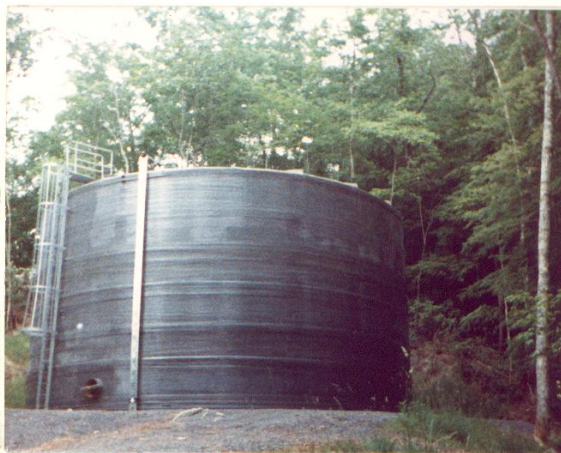
200,000 gallon potable water storage vessel, Field fabricated by Plas-Tanks Industries, Inc. In Great Smoky Mountain National Park
